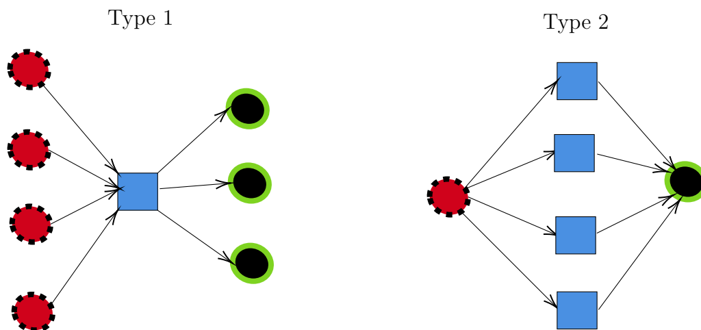
Fig. 1. Type 1 (left) and type 2 (right) smurf-like motifs. Source (red dotted circles), middle (squares), and target (green circles) are shown from left to right.
