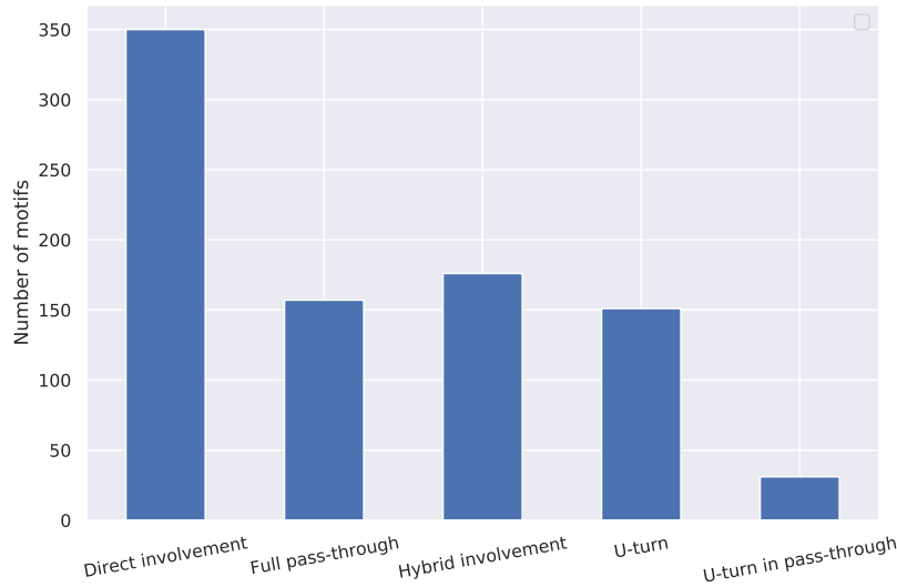
Fig. 4. Number of motifs extracted from the whole data set for each class, defined in the main text.
